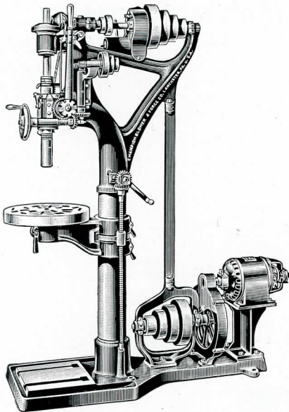
22"—Gear Driven
