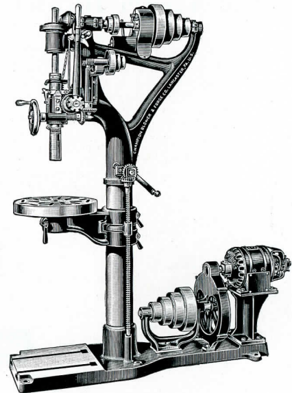
20"—Gear Driven
