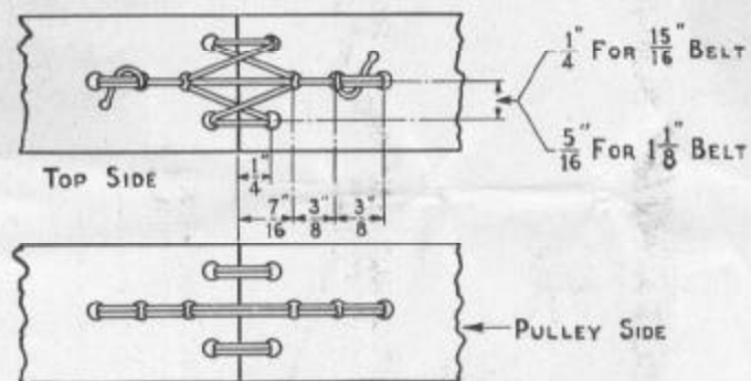
Fig. 11. Spacing of holes for \frac{15}{16} " and 1\frac{1}{8} " belts.
